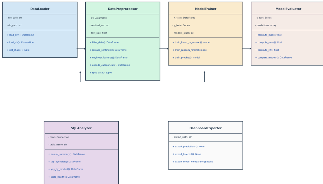
Figure 4.2: Class Diagram
